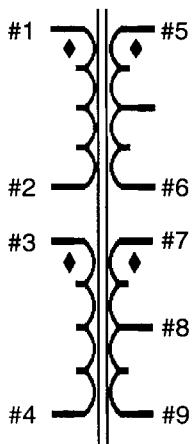
ROX HTX 5099 Transformer
